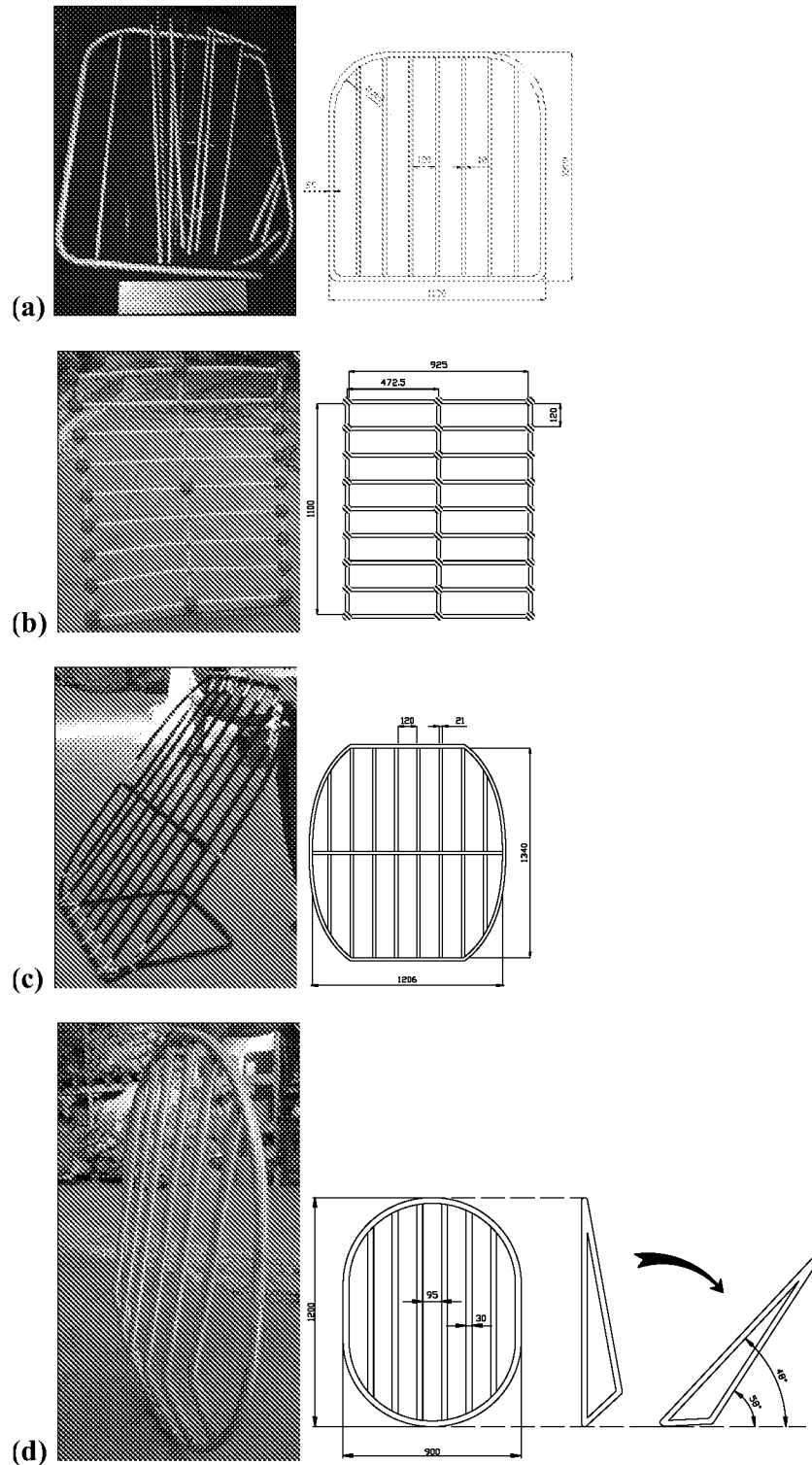
Fig. 2. Dimensions (mm) of the Turtle Excluder Devices (TED): (a) TED1, made of aluminium. The bars were removable to enable the adjustment of the space between them. TED1 broke down because of the large quantity of debris. (b) TED2, made of a flexible grid of mixed cable (steel inside and polyethylene outside). TED2 was installed with the aim of making the TED position capable of adjusting according to net movements during tow. (c) TED3, made of a semi-rigid and resistant grid of steel and rubber, with the aim of combining the flexibility of rubber and the resistance of steel. (d) TED4, the Supershooter grid made of classic aluminium. TED4 is commonly used in prawn fisheries in several countries. To take into account the complex fishing composition (crustaceans, molluscs and fishes together), we kept the space between reflector bars larger than in the standard models.
