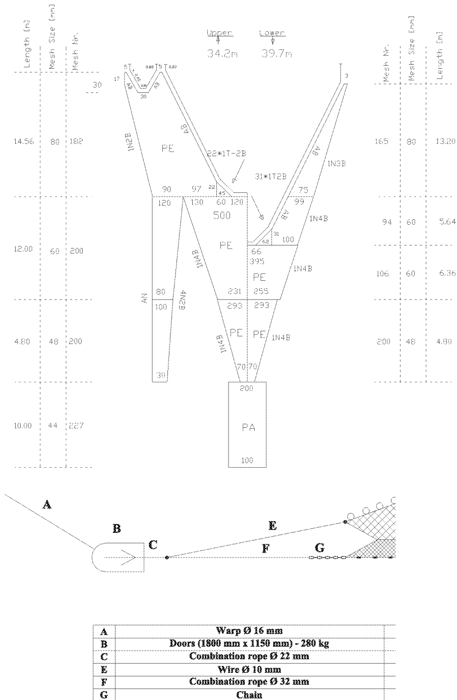
Fig. 1. Design and gear rigging of the trawl used during the samplings at sea. The trawl is a 4-faced bottom trawl, recently introduced in the Adriatic Sea. Apart the polyamide codend it is entirely made of knotted polyethylene (PE) netting.
